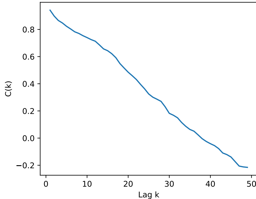
LUMO Autocorrelation
