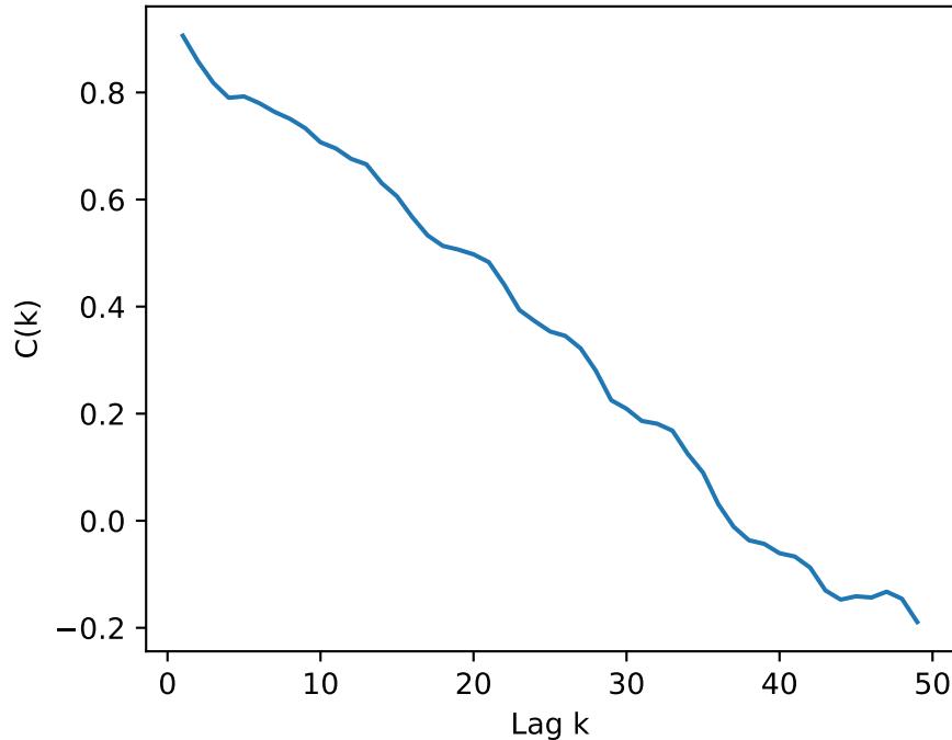
HOMO Autocorrelation
